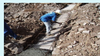
Jozini High School strip footing
